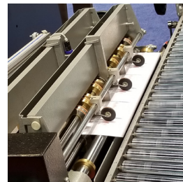
Strike-slit feature
